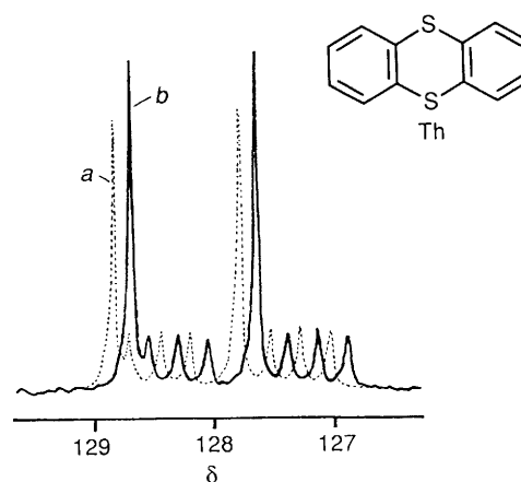
Fig. 2 Proton-decoupled ^{13}\text{C} NMR spectra of the \alpha - and \beta -carbons of Th and [\text{}^2\text{H}_8]\text{Th} taken in \text{CDCl}_3 from: (a) a mixture consisting of [\text{}^2\text{H}_8]\text{Th}]:[\text{Th}] = 1.00 ; (b) the same mixture after 50% oxidation with perchloric acid and removal of the radical cations formed. Both spectra were recorded on a Bruker AM 400 NMR spectrometer at 100.6 MHz under identical conditions and a very long pulse delay was used to ensure the complete relaxation of the deuterium attached carbons (9.2 \mu\text{s} pulse width, 20 s pulse delay, same decoupling and lock power).
